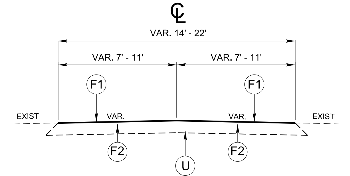
TYPICAL SECTION NO. 1 MAPS # 1 - 4, 6, 8, 11, 13 - 16, 22 - 28, & 30 - 71
