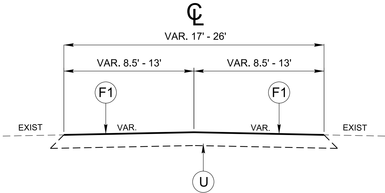
TYPICAL SECTION NO. 3 MAPS # 9 - 10, 12, 17 - 21, & 29
