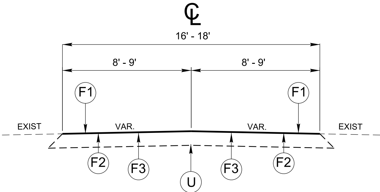
TYPICAL SECTION NO. 2* MAPS # 5 & 7
